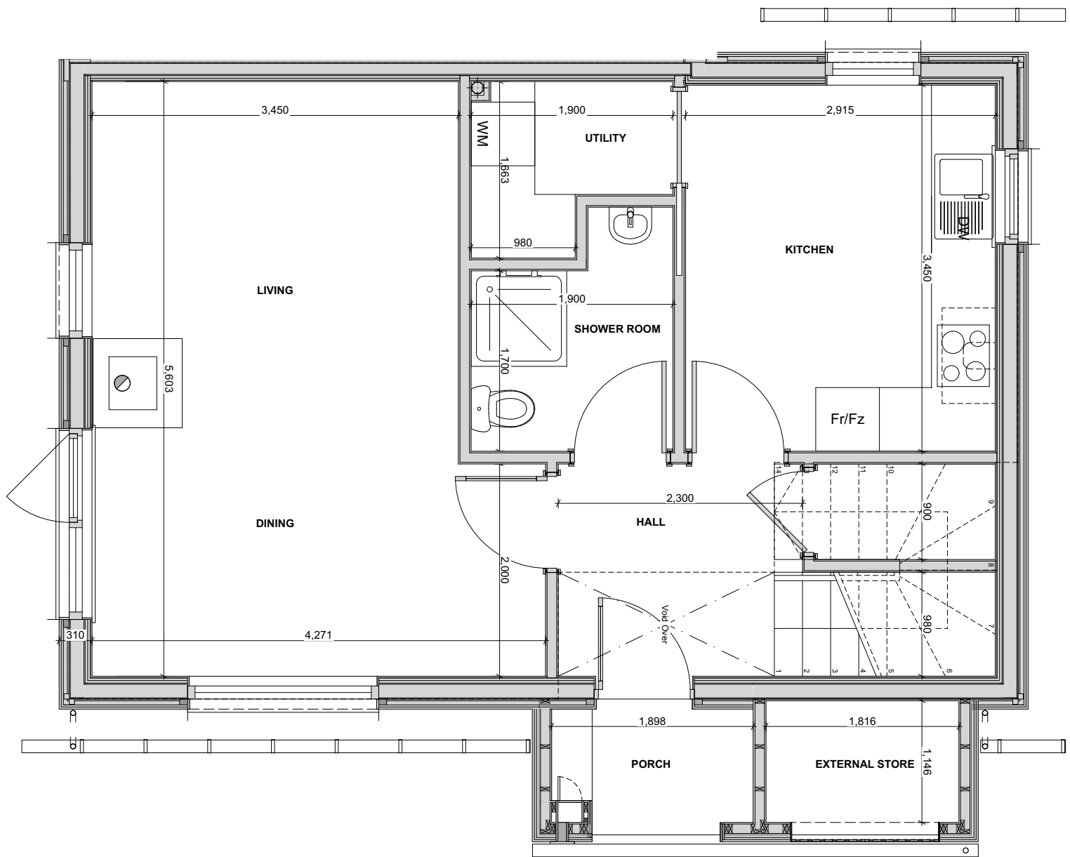
Block E - 3 Bedroom Ground Floor Plan 1:50
