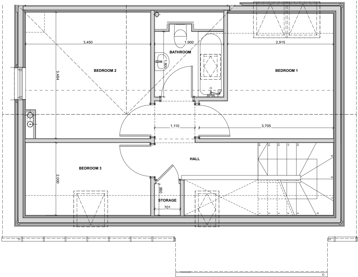
Block E - 3 Bedroom First Floor Plan 1:50
