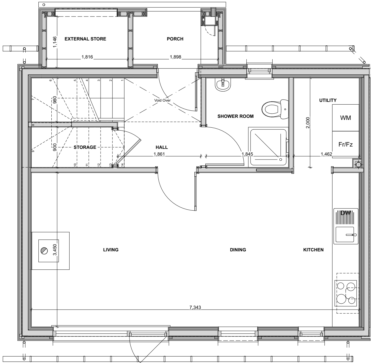
Block E - 2 Bedroom Ground Floor Plan 1:50
