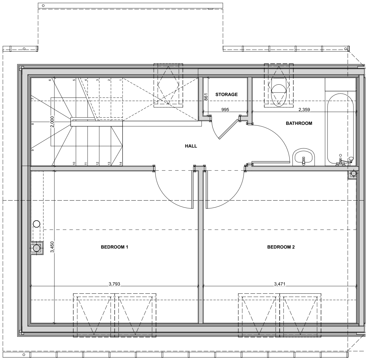
Block E - 2 Bedroom First Floor Plan 1:50
