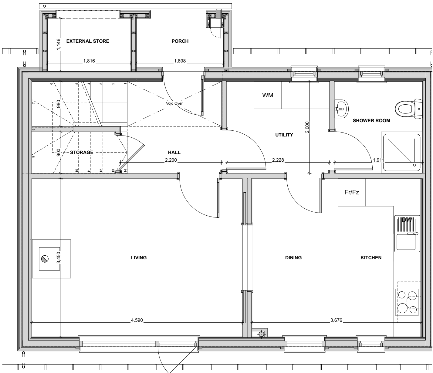
Block D - 3 Bedroom Ground Floor Plan 1:50
