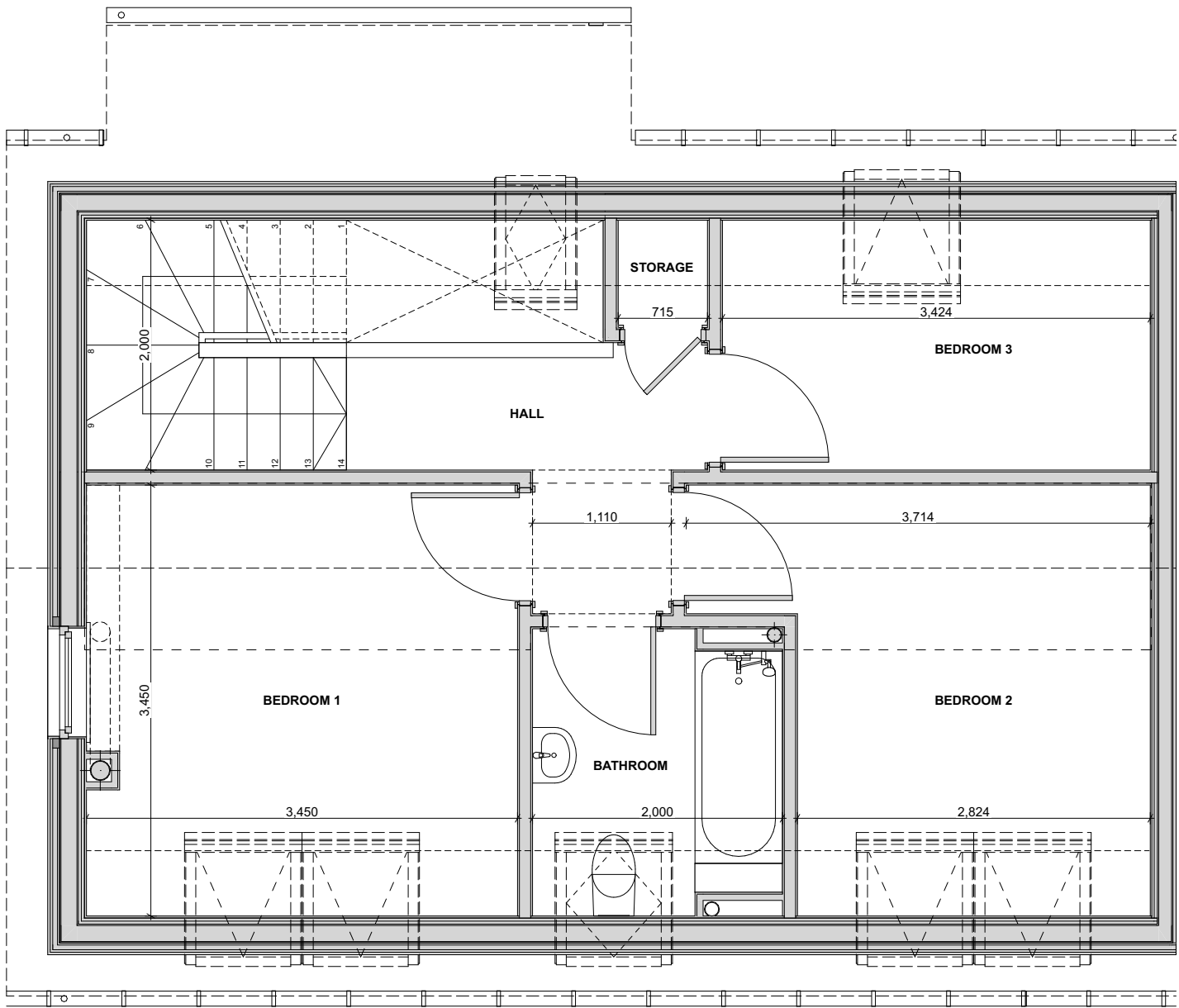
Block D - 3 Bedroom First Floor Plan 1:50
