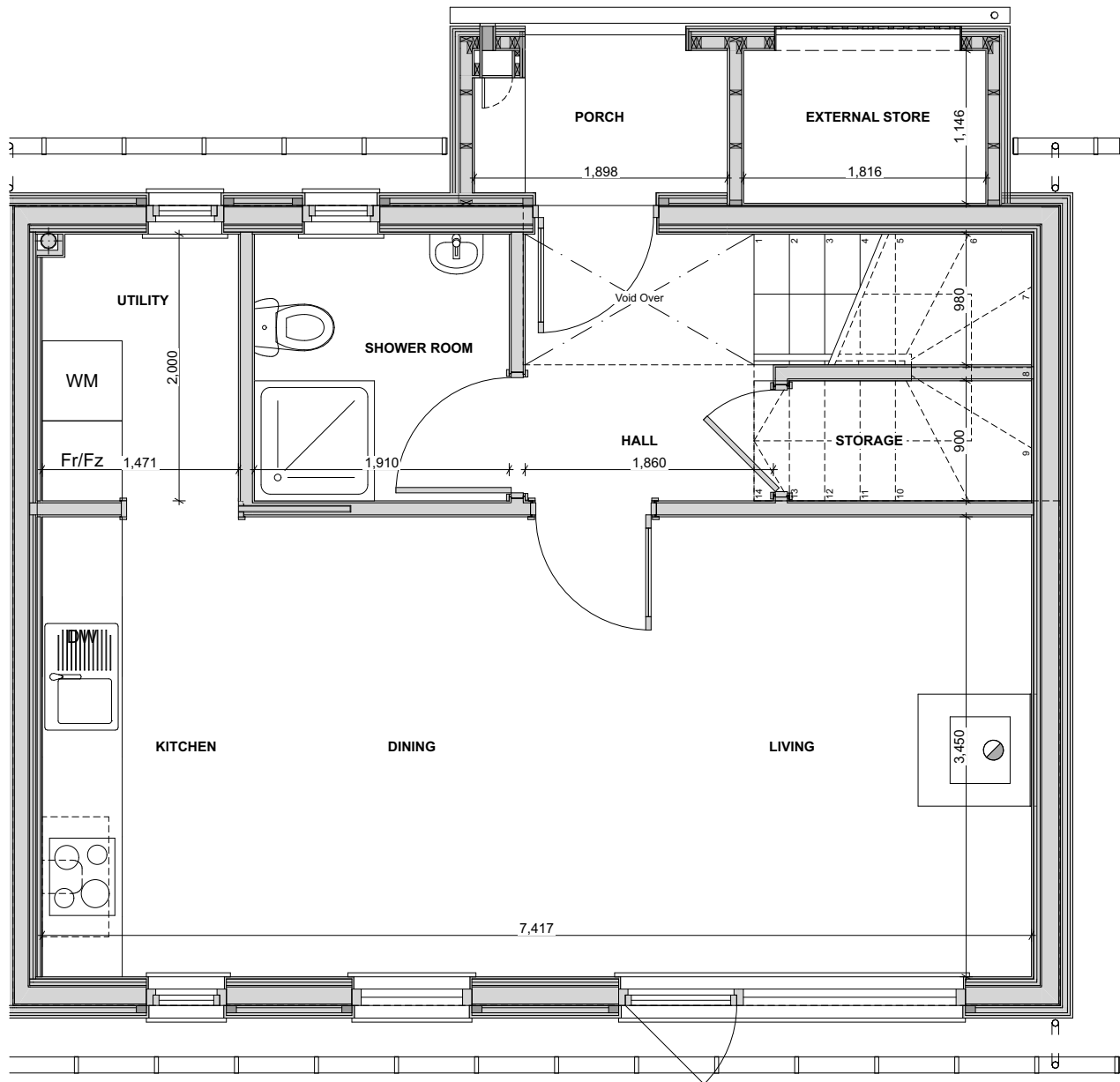
Block D - 2 Bedroom Ground Floor Plan 1:50
