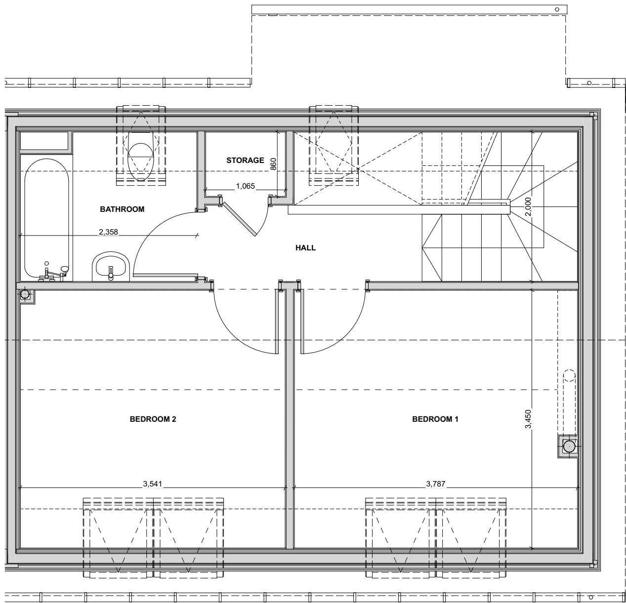
Block C - 2 Bedroom Ground Floor Plan North 1:50
