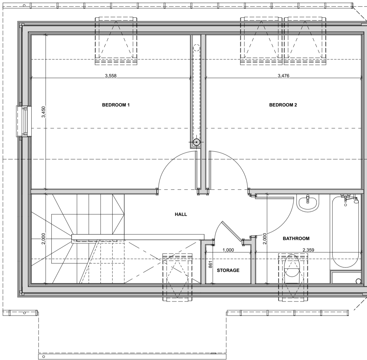
Block B - 2 Bedroom Ground Floor Plan 1:50
