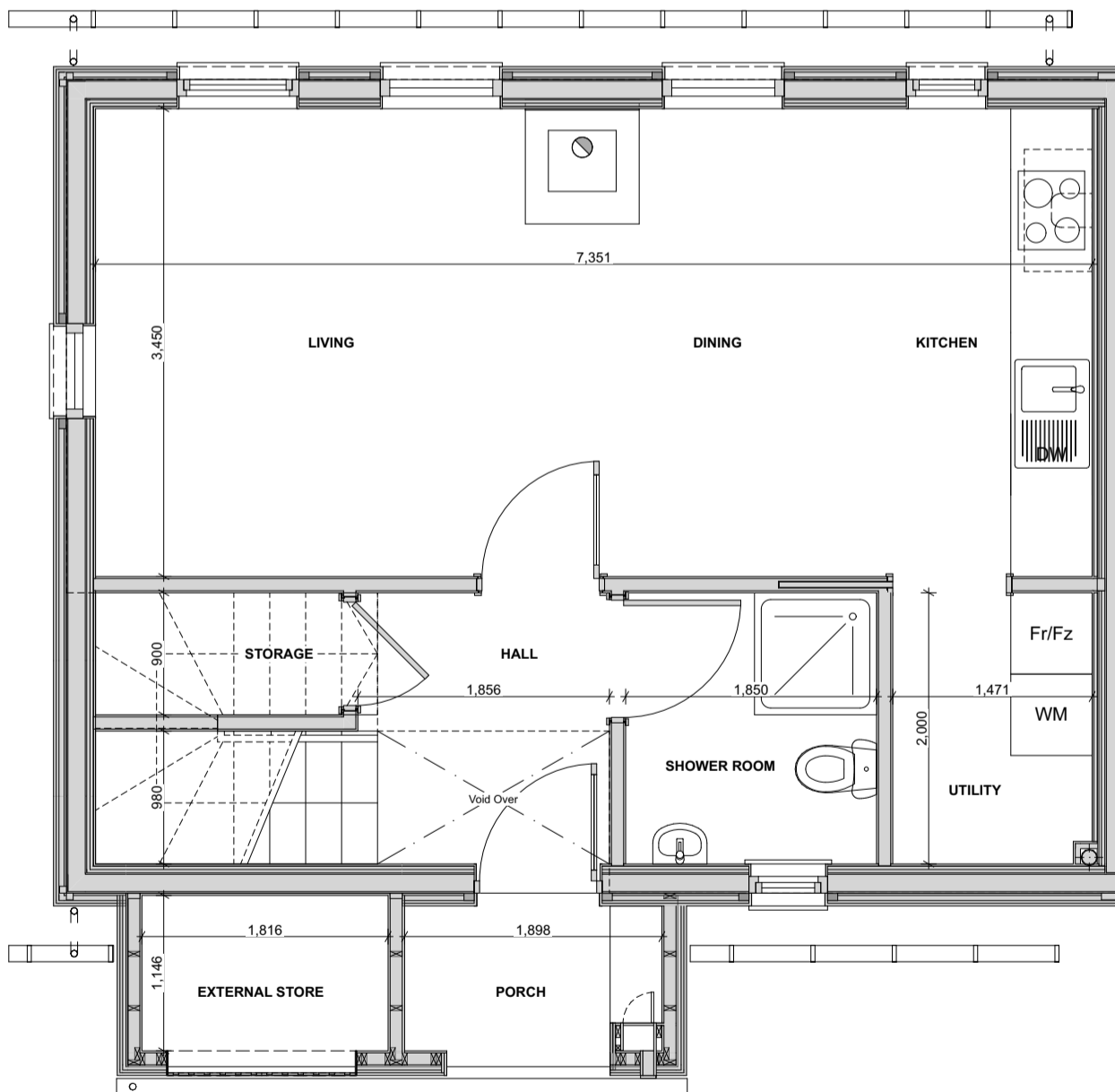
Block B - 2 Bedroom Ground Floor Plan 1:50
