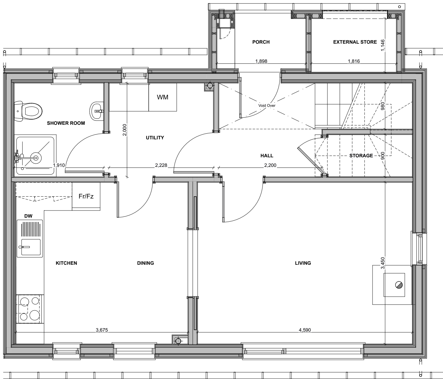
Block A - 3 Bedroom Ground Floor Plan 1:50
