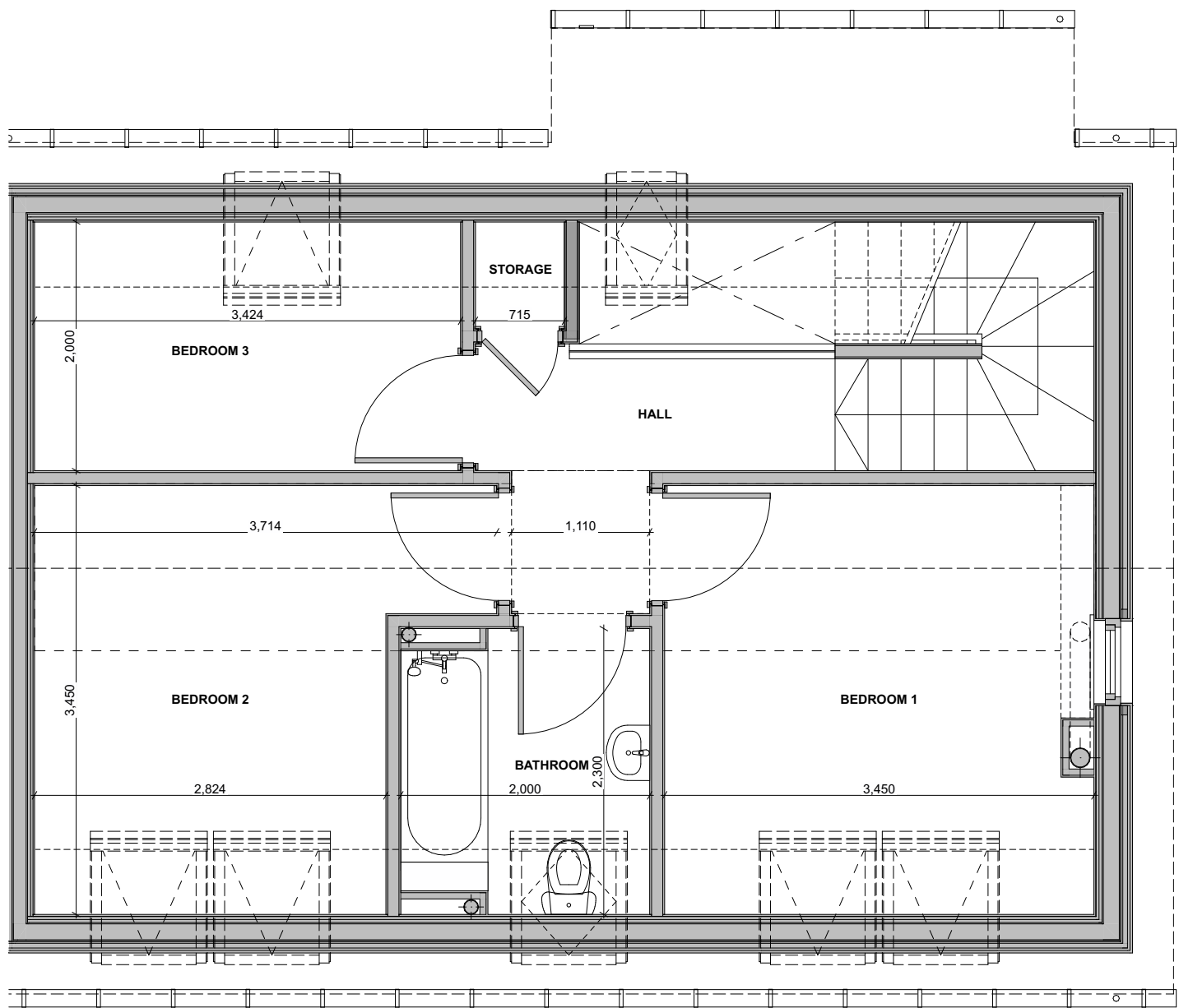
Block A - 3 Bedroom First Floor Plan 1:50
