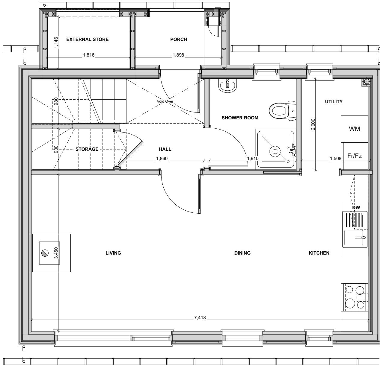
Block A - 2 Bedroom Ground Floor Plan 1:50
