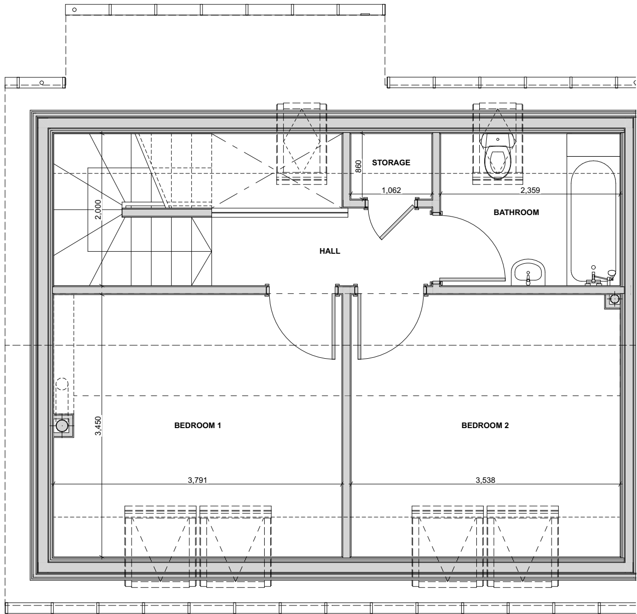
Block A - 2 Bedroom First Floor Plan 1:50
